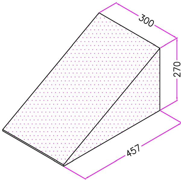
SLOPING TOP FOR INDIVIDUAL LOCKER
